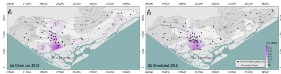
Fig. 1. (a) Location of the study area, main aquifer systems and (a) observed and (b) simulated hydraulic head and concentration of NO 3 in 2013.
