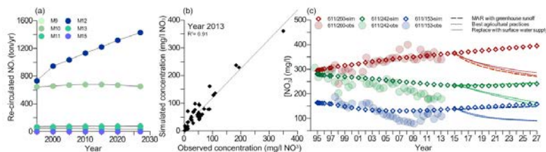
Fig. 2. (a) Rate of re-circulation per aquifer system; (b) observed versus simulated \text{NO}_3 concentrations in 2013; (c) observed and simulated time series of \text{NO}_3 concentration at selected monitoring points (location in Fig.1(b)).
