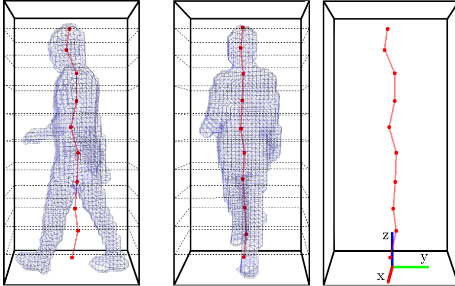
Figure 2: The reconstructed model is divided into 3D stacked areas of the same size called slices (regions within dotted lines). Centroids are computed on each slice (red points). The gait feature is composed by a set of inner angles between the line joining each pair of consecutive centroids (red line) and the z-axis in R3. Best viewed in color.
