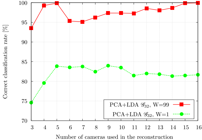
Figure 11: Performance of our descriptor on KY4D database for an increasing number of cameras.
