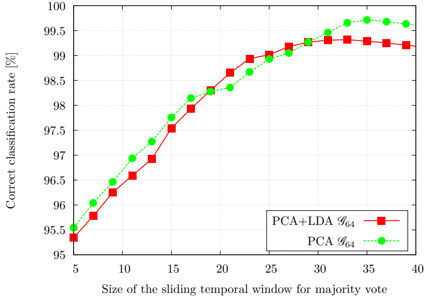
Figure 9: Performance of our descriptor on the AVAMVG database for different lengths of the majority voting window.
