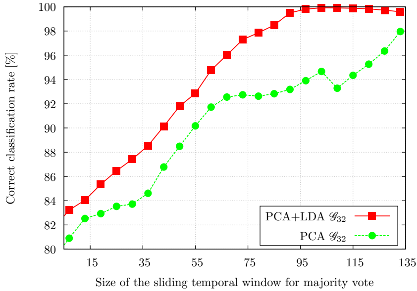
Figure 10: Performance of our descriptor on the KY4D database for different lengths of the majority voting window.
