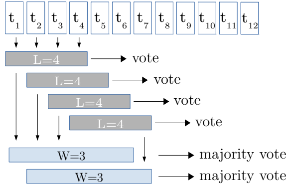
Figure 5: Majority vote policy over a sliding temporal window. In the example, the size of the signature is set to L=4 , and the size of the voting window is set to W=3 .
