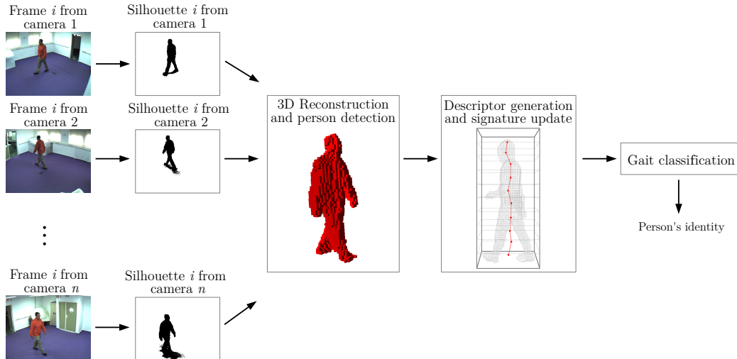
Figure 3: Pipeline of our approach.
