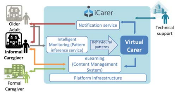
Figure 1: iCarer platform
