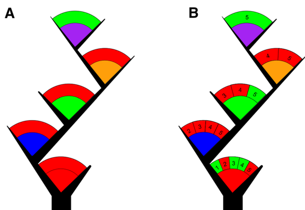
Fig. 4 a Test-based tree illustrating pairwise comparisons between the branch orders in layers IIIPost and VPost. If the arc that appears above the branch order color code is red , the test produced a rejection result. If the arc is green , the result was non-rejection. b Comparisons of branch-order angles grouped according to their maximum branch order. The numbers in the arc above the branching color codes indicate the maximum tree order and each of the subdivisions of the arc corresponds to a test. As an example, the first branch order in the graphic shows the information of five tests performed to the first branch order of dendrites with maximum tree orders 1, 2, 3, 4, and 5
