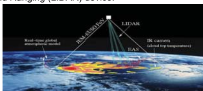
Figure 1: Scheme of the Atmospheric Monitoring System.
