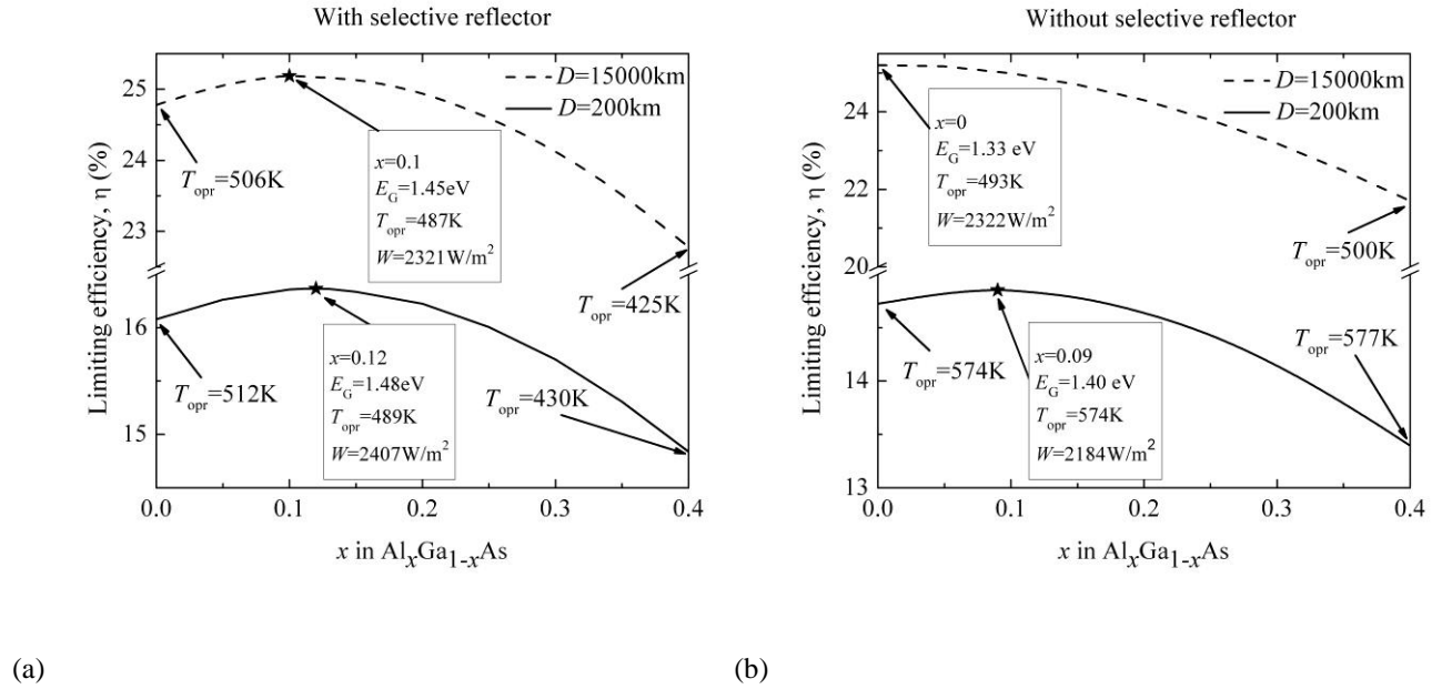
Fig. 2. Limiting efficiency of solar cells based on Al_xGa_{1-x}As with ideal selective reflectors (a) and without selective reflectors (b).
