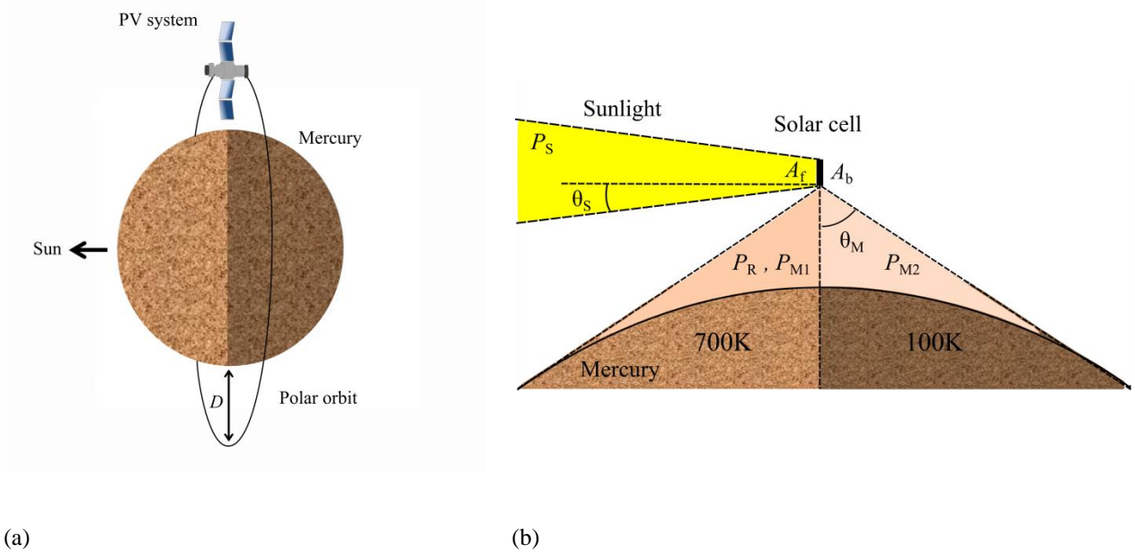
Fig. 1. (a) Sketch of the polar orbits around Mercury that are studied in this work. (b) Side view of the different power radiations received by the solar cells.
