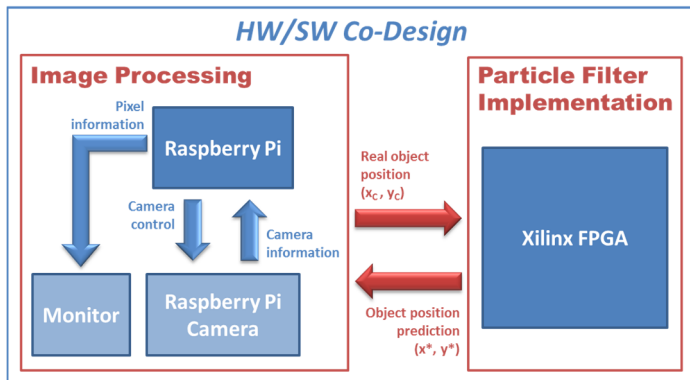
Fig. 3. System architecture.
