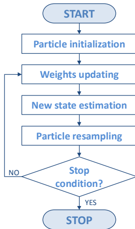
Fig. 1. Basic particle filter flowchart.
