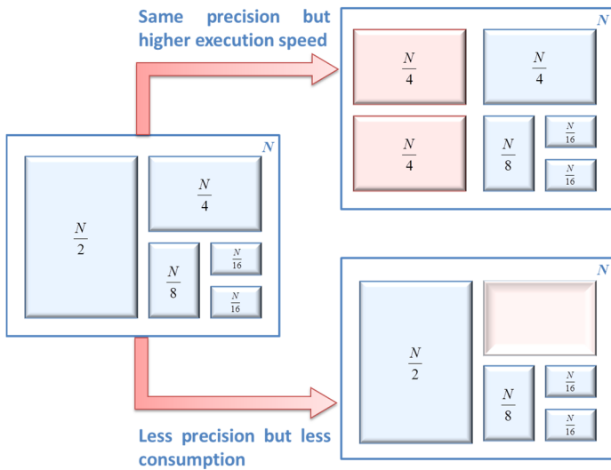
Fig. 2. Adaptive modular division of the particle filter.
