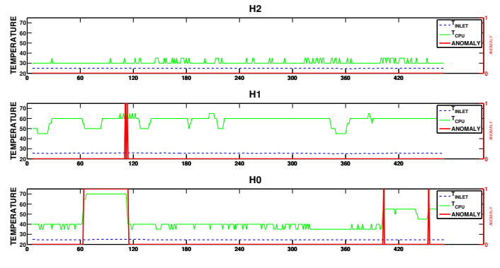
Fig. 6. Contextual anomaly in H0 starting around tick 65
