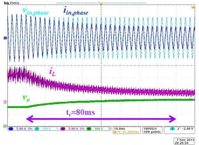
Fig. 13. Measurement of energy loop working under power load step from 1.8kW down to 650W, i_{in} is controlled to vary smoothly and consequently causes v_o to increase slowly from 150V to 220V. V_{in,phase} [100V/div], i_{in,phase} [5A/div], i_L [5A/div], v_o [100V/div].
