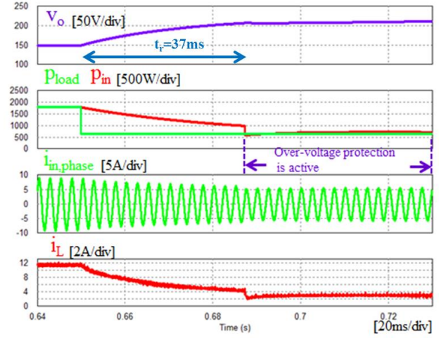
Fig. 9. Transient response for switching model simulation applying over-voltage protection.
