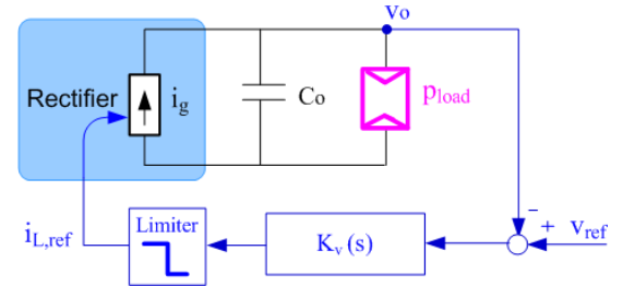
Fig. 5. Simplified model of a current controlled buck rectifier with conventional outer voltage loop.
