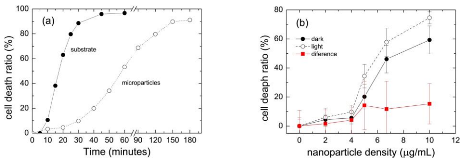
Figure 7: (a) Time evolution of the fraction of dead cells evaluated through morphological criteria for tumor cells cultured on Fe:LiNbO 3 substrates (solid circles) or in contact with Fe:LiNbO 3 microparticles (open circles). (b) Fraction of dead cells vs Fe:LiNbO 3 nanoparticle density under illumination (open circles) and in dark (solid circles). The difference between both curves is also represented (red solid squares).
