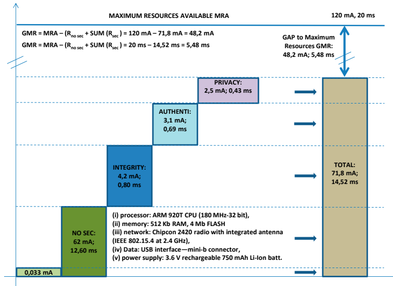
Figure 2. Energy spent vs. security services, and delay vs. security services.
