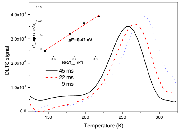
Figure 5: DLTS spectra for a GaAs device. Three rate windows were used; the corresponding Arrhenius plot is in the inset. The defect energy obtained is 0.42eV (respect to the valence band).
