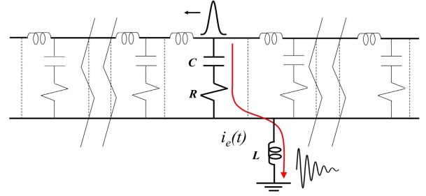
Figure 3. Equivalent RLC circuit to simulate damped sinusoidal waveforms.
