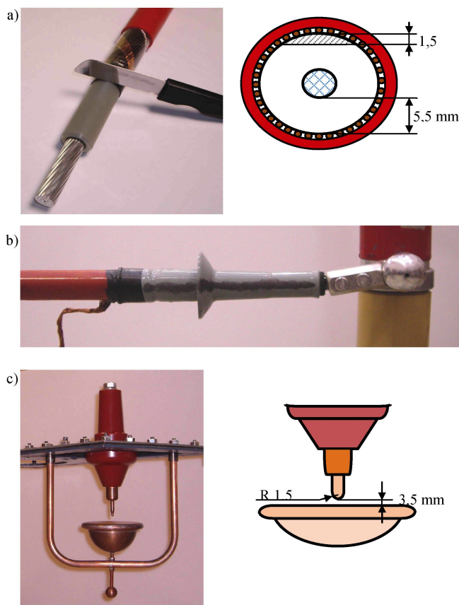
Figure 9. PD sources. a) Cavity in a cable termination, b) surface insulation defect and c) point-plane corona effect.
