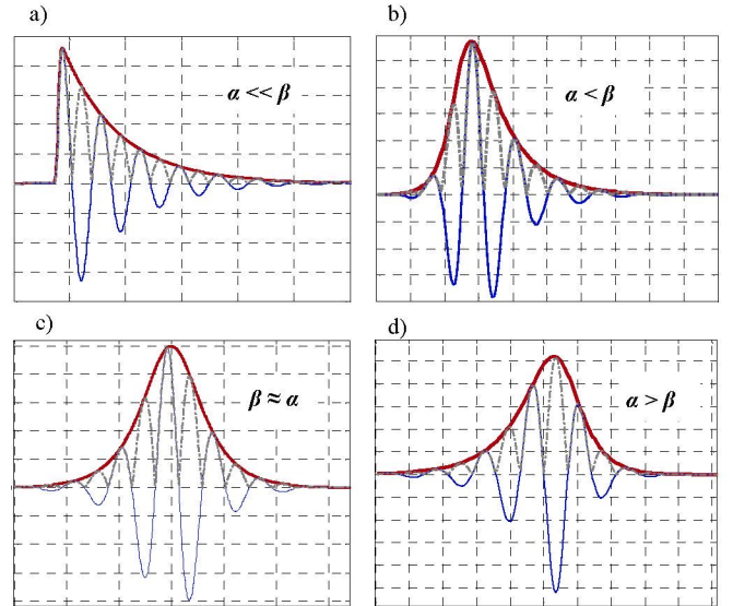
Figure 6. Enveloping functions for different types of pulses. a) Asymmetric pulse skewed to the left with the maximum value in the first peak. b) Asymmetric pulse with an oscillation before the maximum value. c) Symmetric pulse. d) Asymmetric pulse skewed to the right.
