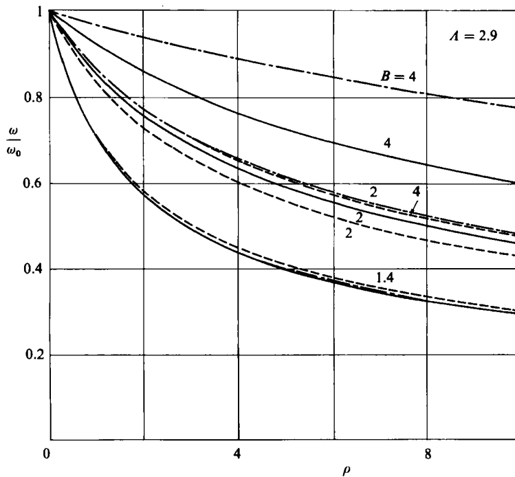
FIGURE 11. (a) Pulsation \omega versus wall position B and (b) pulsation versus density ratio \rho , compared with non-surrounded liquid-bridge pulsation \omega_0 . First oscillation mode of a surrounded bridge of slenderness A . Results obtained from several linearized models: three-dimensional (solid line), infinite columns (dashed line) and one-dimensional (dot-dashed line).
