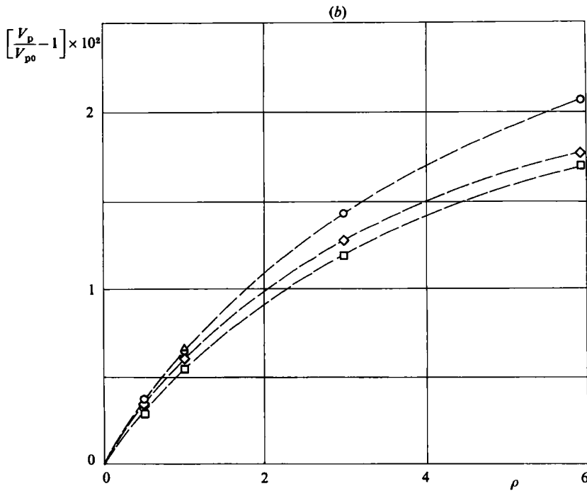
FIGURE 3. Variation of the partial breaking volume V_p of a surrounded liquid bridge, (a) with the wall position B and (b) with the density ratio \rho , compared with that of a non-surrounded bridge V_{p0} of the same slenderness A and initial perturbation \epsilon . (a) \rho = 1 ; (b) B = 2 . Symbols are defined in table 1.
