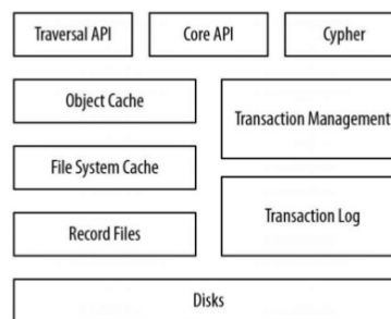
Figure 1: Neo4j Architecture
