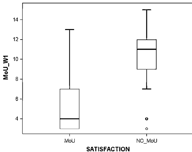
Fig. 12. Box and whisker plot for User satisfaction level with and without MoU1_W.
