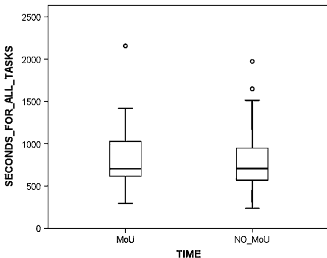
Fig. 13. Box and whisker plot for Time to finish the tasks with and without MoUs.
