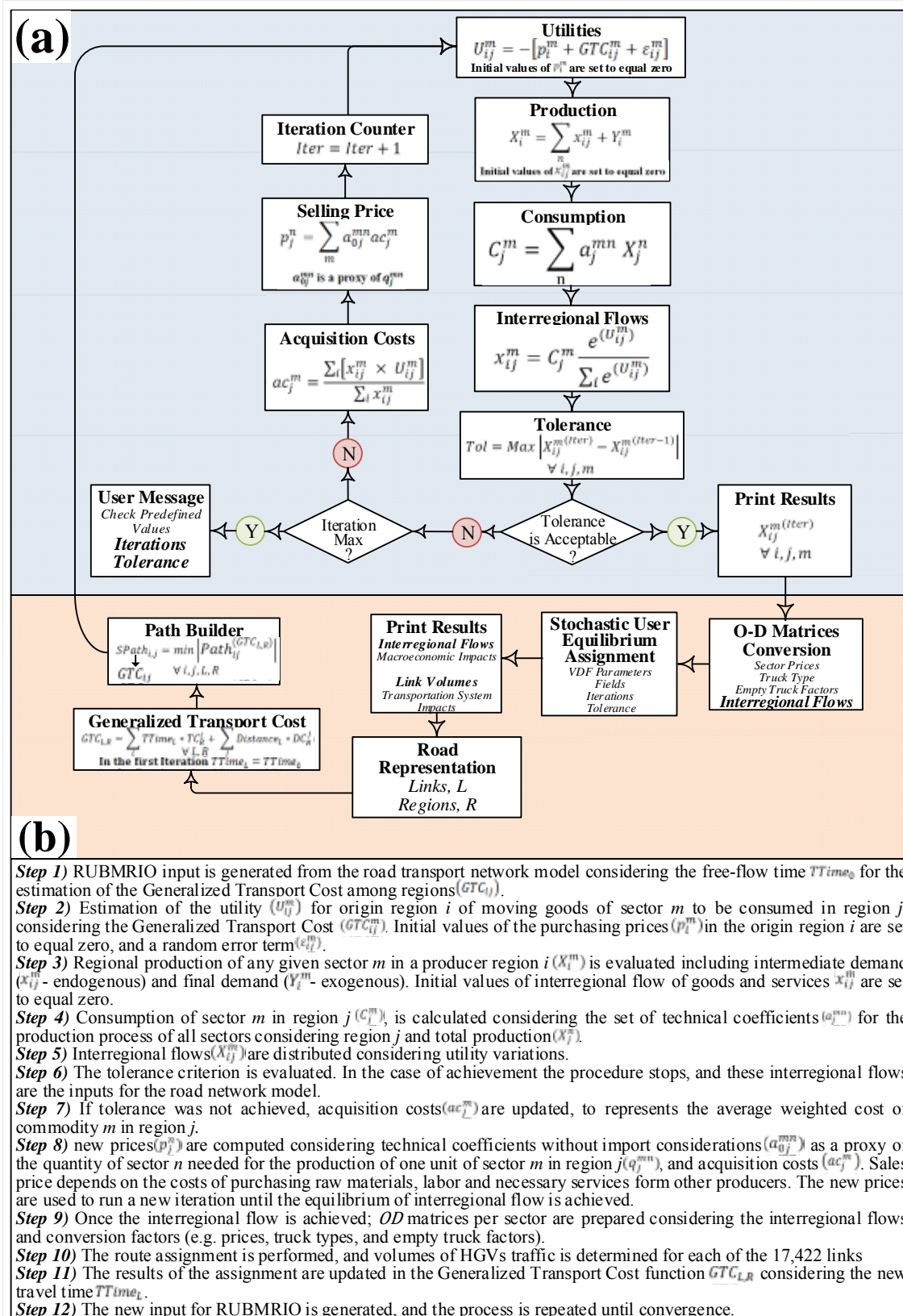
Fig. 1 – An Integrated Approach for Transportation Impact Assessment: (a). RUBMRIO Algorithm; (b) the Road Transport Network Model
