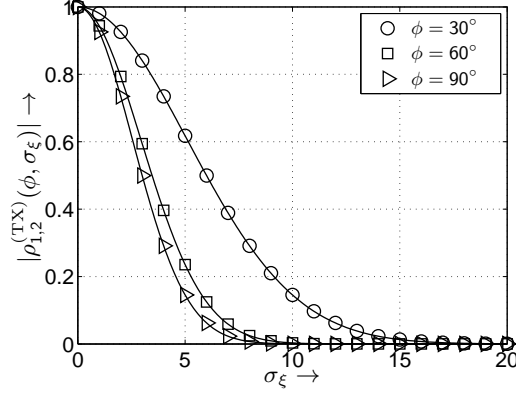
Fig. 3. Variation of the correlation coefficient |\rho_{1,2}^{(\text{TX})}(\phi, \sigma_\xi)| as a function of \sigma_\xi and \phi assuming a wavelength specific antenna separation of d_\lambda = 1/16
