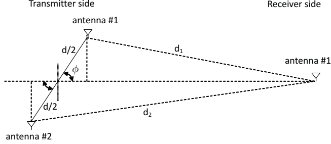
Fig. 1. Antennas' physical disposition: two transmit and one receive antennas
