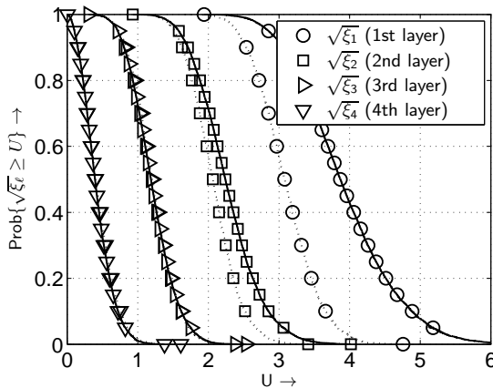
Fig. 8. CCDF of the layer-specific distribution for weakly correlated (solid line) as well as uncorrelated (dotted line) frequency non-selective ( 4 \times 4 ) MIMO channels ( d_\lambda = 1 , \phi = 30^\circ and \sigma_\xi = 1,0 )
