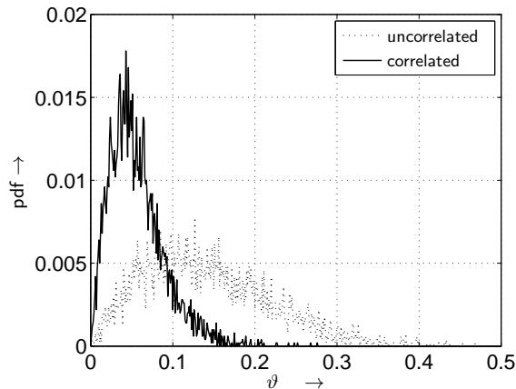
Fig. 7. PDF (probability density function) of the ratio \vartheta between the smallest and the largest singular value for strongly correlated (solid line) as well as uncorrelated (dotted line) frequency non-selective ( 4 \times 4 ) MIMO channels ( d_\lambda = 1/4 , \phi = 30^\circ and \sigma_\xi = 1,0 )
