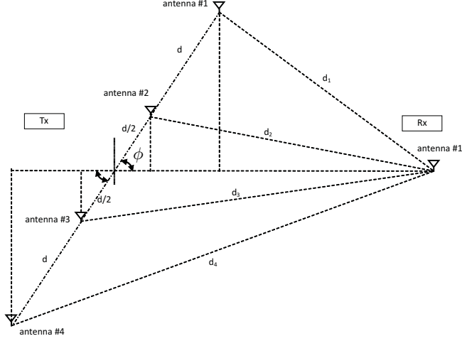
Fig. 4. Antennas’ physical disposition: four transmit and one receive antennas
