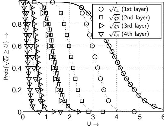
Fig. 9. CCDF of the layer-specific distribution for strongly correlated (solid line) as well as uncorrelated (dotted line) frequency non-selective ( 4 \times 4 ) MIMO channels ( d_\lambda = 1/4 , \phi = 30^\circ and \sigma_\xi = 1,0 )
