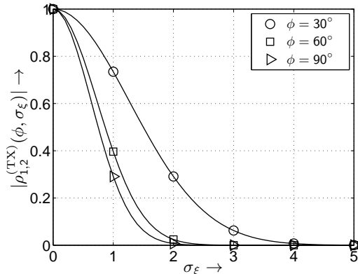
Fig. 2. Variation of the correlation coefficient |\rho_{1,2}^{(TX)}(\phi, \sigma_\xi)| as a function of \sigma_\xi and \phi assuming an antennas separation in wavelengths of d_\lambda = 1/4
