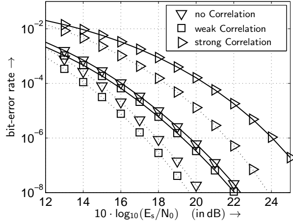
Fig. 13. BER with optimal PA (dotted line) and without PA (solid line) when using the (16, 16, 0, 0) QAM transmission mode and transmitting 8 bit/s/Hz over frequency non-selective ( 4 \times 4 ) MIMO channels with different degrees of correlation
