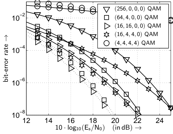
Fig. 11. BER with optimal PA (dotted line) and without PA (solid line) when using the transmission modes introduced in Tab. 2 and transmitting 8 bit/s/Hz over frequency non-selective ( 4 \times 4 ) MIMO channels ( d_\lambda = 1 , \phi = 30^\circ and \sigma_\xi = 1,0 ) with weak transmitter-side correlation
