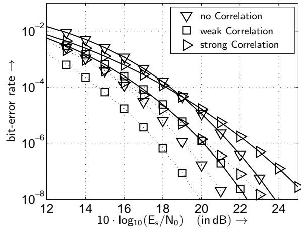
Fig. 14. BER with optimal PA (dotted line) and without PA (solid line) when using the (64, 4, 0, 0) QAM transmission mode and transmitting 8 bit/s/Hz over frequency non-selective ( 4 \times 4 ) MIMO channels with different degrees of correlation
