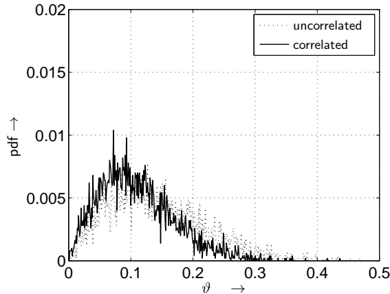
Fig. 6. PDF (probability density function) of the ratio \vartheta between the smallest and the largest singular value for weakly correlated (solid line) as well as uncorrelated (dotted line) frequency non-selective ( 4 \times 4 ) MIMO channels ( d_\lambda = 1 , \phi = 30^\circ and \sigma_\xi = 1,0 )
