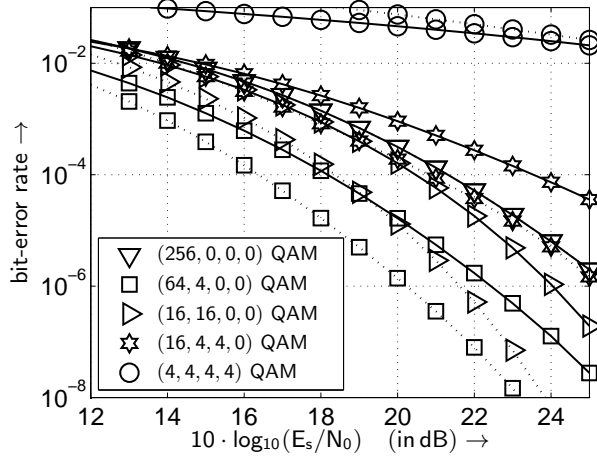
Fig. 12. BER with optimal PA (dotted line) and without PA (solid line) when using the transmission modes introduced in Tab. 2 and transmitting 8 bit/s/Hz over frequency non-selective ( 4 \times 4 ) MIMO channels ( d_\lambda = 1/4 , \phi = 30^\circ and \sigma_\xi = 1,0 ) with strong transmitter-side correlation
