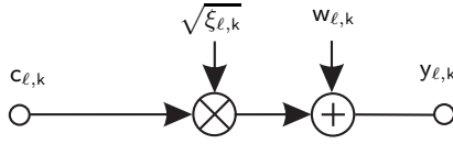
Fig. 5. Resulting system model per MIMO layer \ell and transmitted data block k
