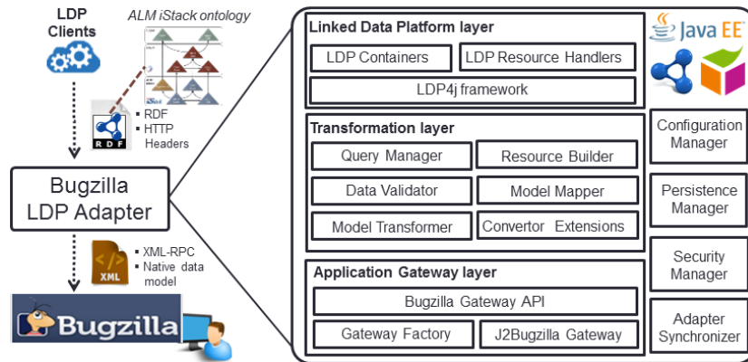
Fig. 1. High-level architecture of the Bugzilla adapter
