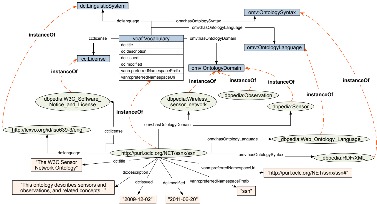
Figure 3: Example of ontology metadata representation in RDF.
