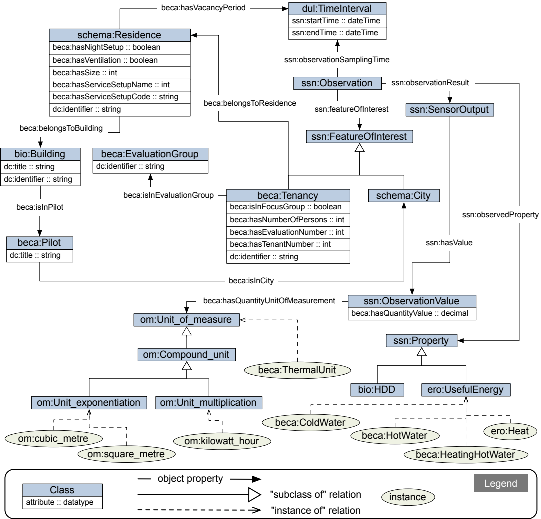
Figure 3. The BECA ontology.
