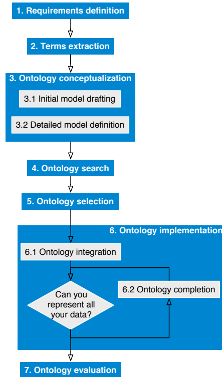
Figure 1. Workflow of activities for ontology development.
