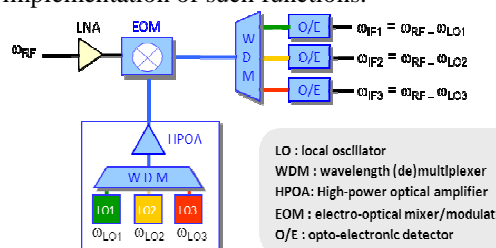
Fig. 2. Optical Multi-Frequency Conversion concept
