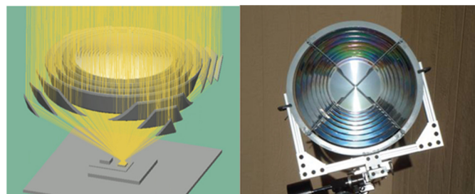
Fig. 12 Ring array concentrator. 56
