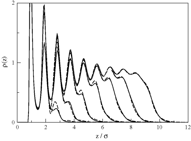
Fig. 4. Density profiles of adsorbed films for the Lennard-Jones fluid close to its triple point. Full lines are simulation results for films of thickness \ell (from left to right) 1.9, 3.0, 4.1, 5.3, 6.5, 7.3 and 8.5 molecular diameters, \sigma . Dashed lines are predictions from the superposition model, Eq. (35). Note that the discontinuity in the first derivative of the density profile is hardly visible. Results adapted from Ref. [45,83] correspond to the same model and temperature as the two preceding figures.
