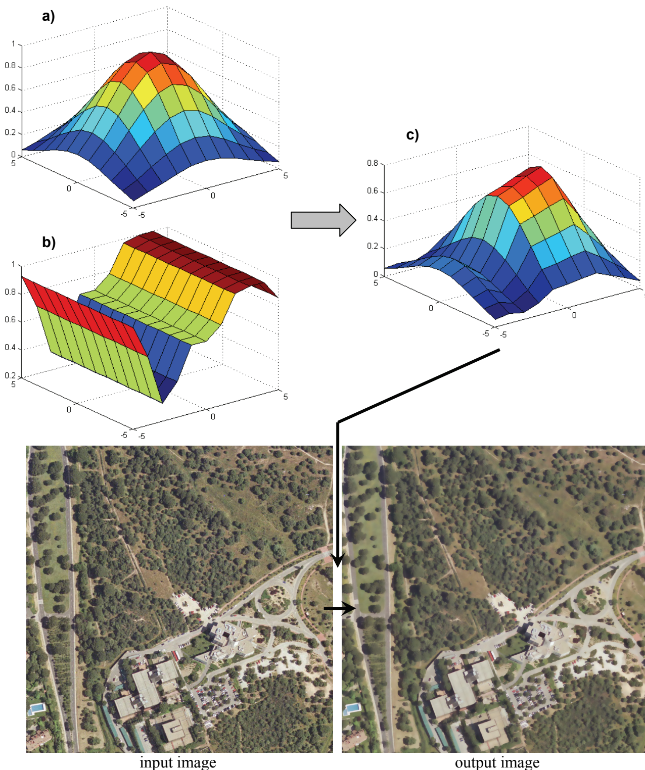
Figure 1: Pre-segmentation bilateral filtering scheme. Domain (a), Range (b) and Bilateral (c) filters.
