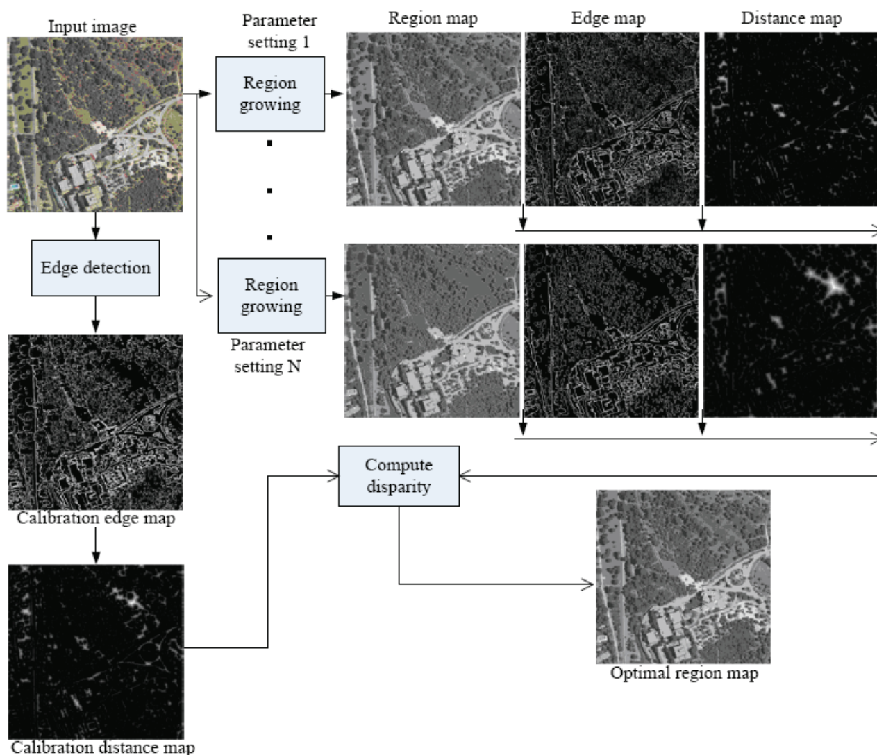
Figure 2: Methodological scheme. The edge information is used to evaluate the quality of a segmentation in order to choose the best segmentation from a set of region-based results.
