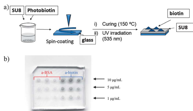
Fig. 5 (a) Scheme of biotinylation procedure incorporated into the SU-8 polymer fabrication. (b) a-BSA and a-biotin microarrays on SU-8-photobiotin 1/1 (v/v) chip. Concentration disposition is in accordance with Fig. 4.
