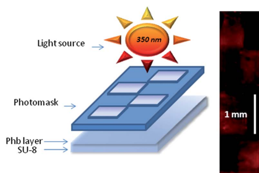
Fig. 4 Fluorescence image obtained after irradiation through a photomask.
