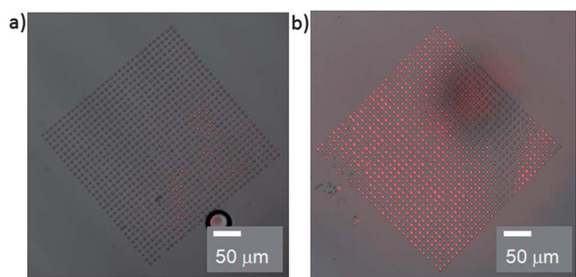
Fig. 7 Confocal image and fluorescence confocal image superposed for an array of nanopillars fabricated in (a) SU-8 and (b) SU-8–Phb 1/1 and incubated with ATTO–streptavidin for 10 minutes.
