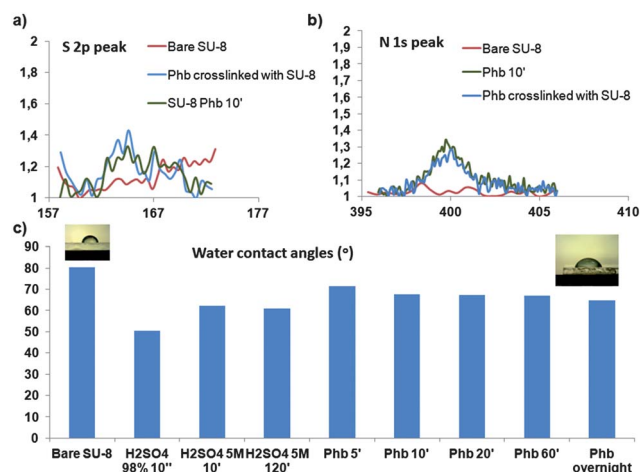
Fig. 2 XPS analysis of (a) the S 2p peak and (b) the N 1s peak for the bare SU-8 surface, the SU-8 polymer coated with photobiotin, and the biotinylated SU-8 surface employing the SU-8 and photobiotin polymerization mixture. (c) Contact angle values for both SU-8, bare and under different hydrolysis and biotinylation conditions.
