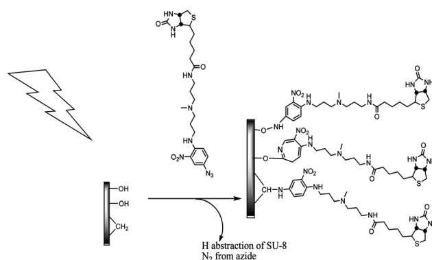
Fig. 1 Photobiotin insertion on the SU-8 polymer under 350 nm light irradiation.
