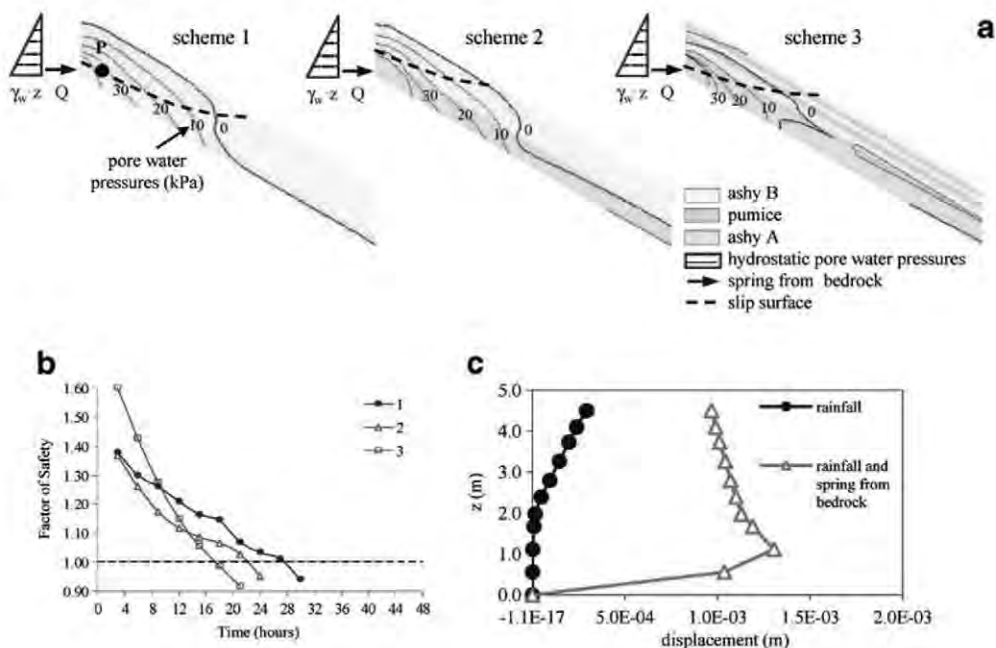
Fig. 7 Failure stage induced by karst springs from bedrock: a pore water pressures simulated at failure, b slope factor of safety (FS) versus time as computed through limit equilibrium analyses and c displacements at vertical passing for point P as simulated via uncoupled stress-strain analyses
