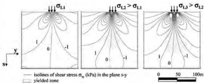
Fig. 10 Stresses variations due to pressures applied at the upper boundary of a plane parallel to ground surface ( y - s plane of Fig. 1)
