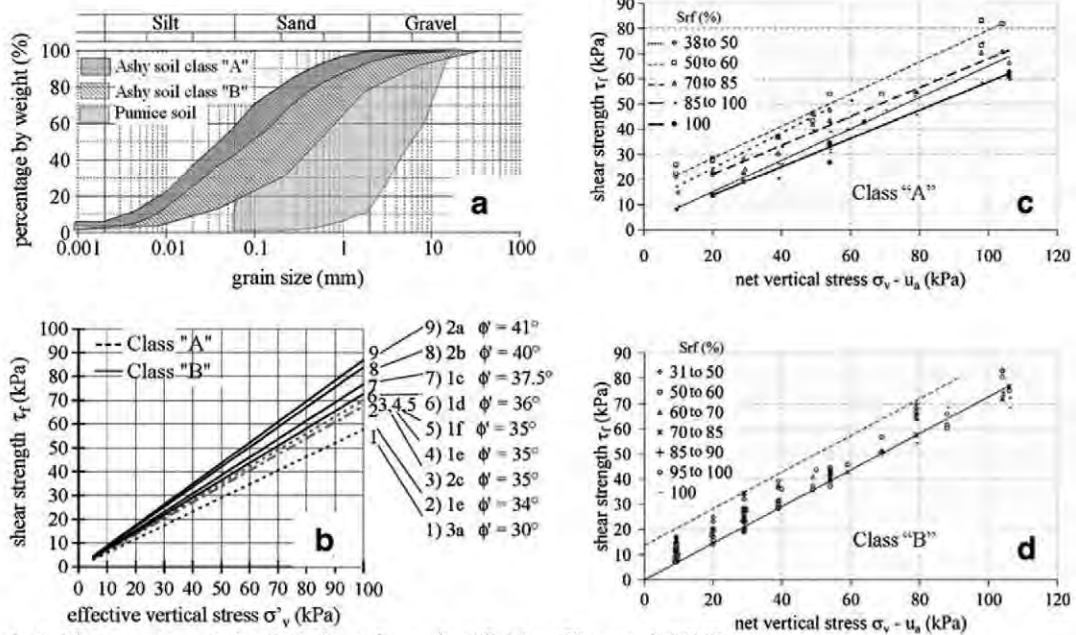
Fig. 6 Main mechanical features of pyroclastic soils in the study area [modified from Bilotta et al. (2005)]
