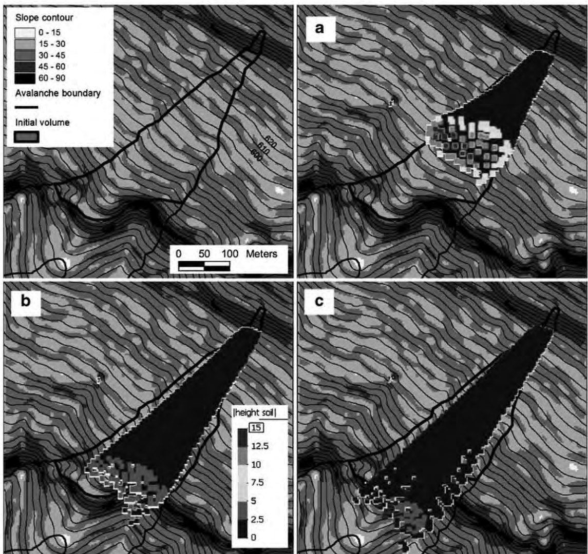
Fig. 11 Topography, initial volume and boundary of observed avalanche source area in the Cortadonica basin (Fig. 4b); Simulated heights of propagating mass with increasing rate of entrainment (a 0.0082, b 0.0012 and c 0.0001) after the same elapsed time ( t=16 s)
