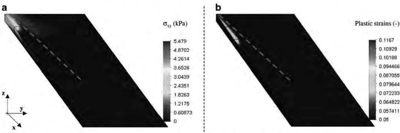
Fig. 9 Hydro-mechanical coupled analysis of impact loading: simulated shear stress in the plane x - y (a) and equivalent plastic strains (b)
