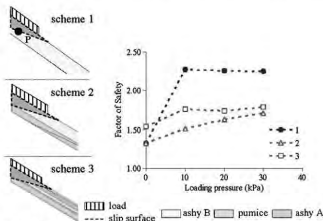
Fig. 8 Effects of a drained loading impact evaluated through the uncoupled limit equilibrium analyses
