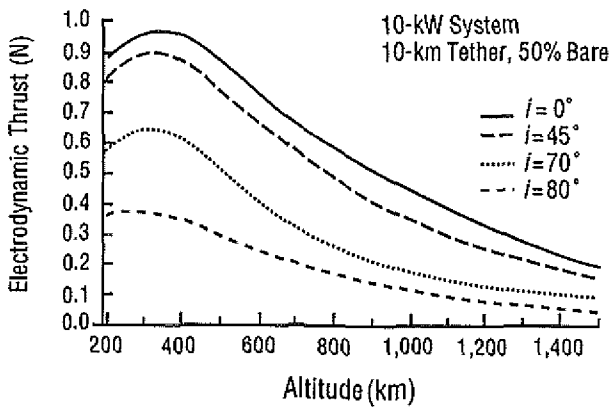
Fig. 6. Performance of an electrodynamic tether thruster.
