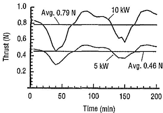
Fig. 5. Comparison of thrust generated for input powers of 5 kW and 10 kW.
