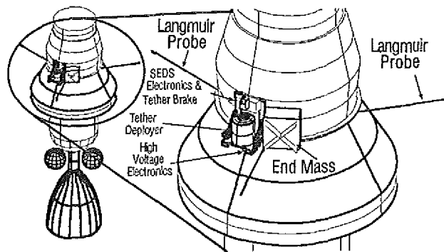
Delta II Second Stage
