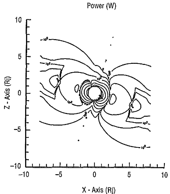
Fig. 8. Power generated in a 10-km tether at Jupiter. Contours are drawn for even decades of power from 1 W to 10 MW.
