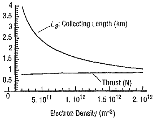
Fig. 2. Variation in thrust with electron density for a 10-km tether with a 5-km-long bare segment.
