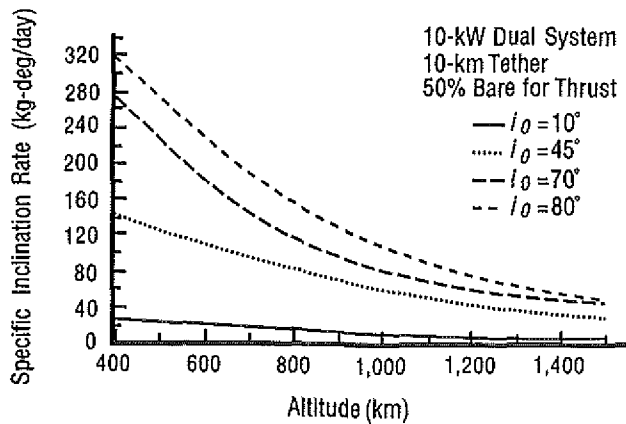
Fig. 7. Electrodynamic tethers change orbital inclination without propellant consumption.
