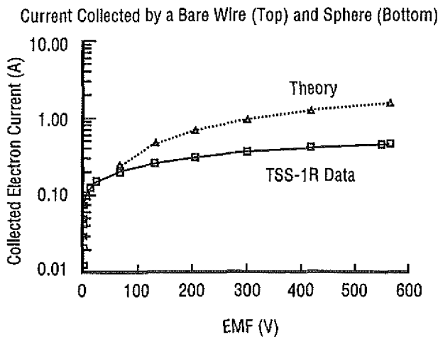
Fig. 1. Current collection efficiency of the bare tether compared to a sphere of equal area.
