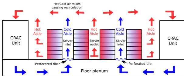
Fig. 1. Data Center cooling scheme
