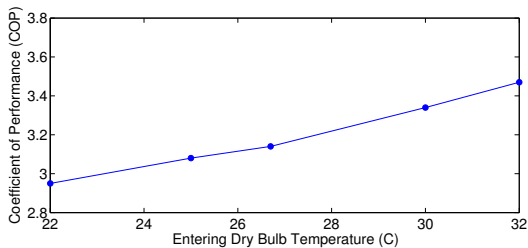
Fig. 2. Evolution of the air-conditioning COP with room temperature
