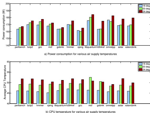
Fig. 5. Power consumption of SPEC CPU 2006 at different air supply temperatures
