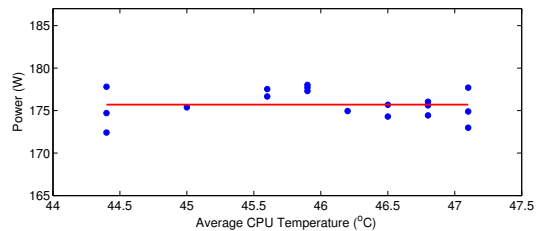
Fig. 3. Power consumption of SunFire V20z for temperature region I
