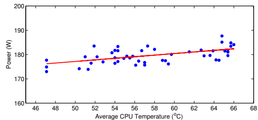
Fig. 4. Power consumption of SunFire V20z for temperature region II
