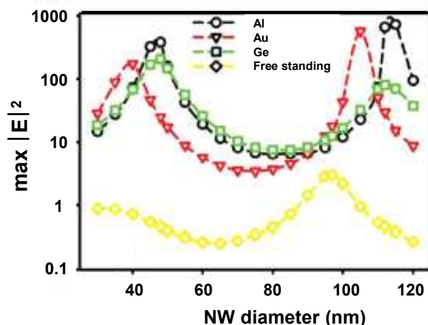
Fig.3. Plot of \max |E|^2 vs the NW diameter using for NWs deposited on different substrates, and also free standing in air
