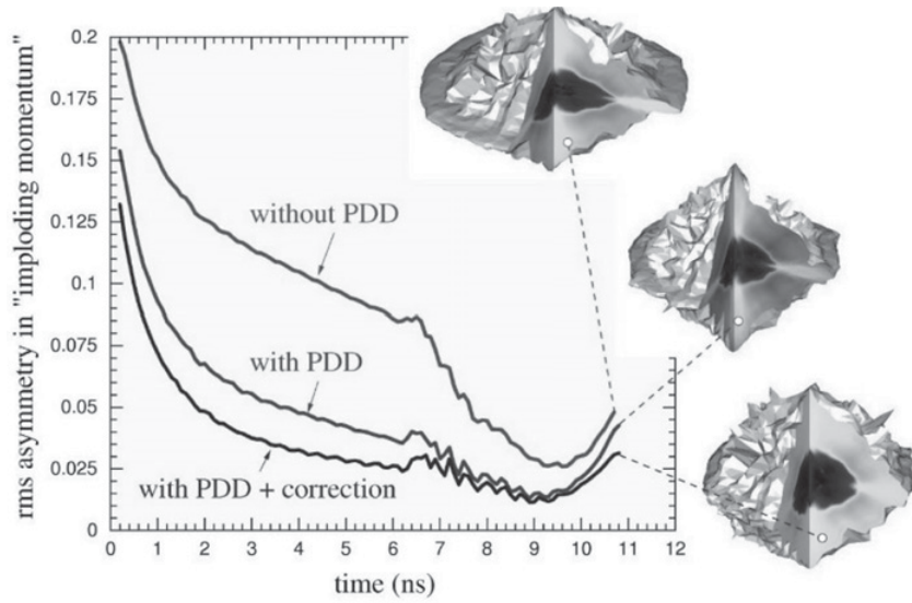
Figure 2. rms distortion for different irradiation schemes as a function of time. Shapes of the shell at the end of each simulation are also shown.
