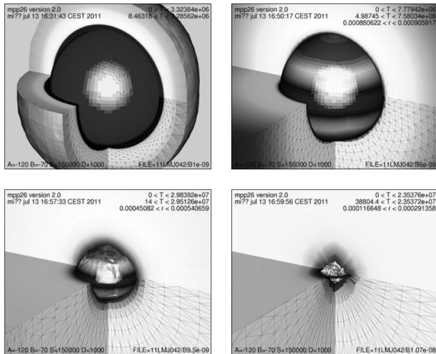
Figure 1. Representative MULTI-3D simulation results of an imploding capsule. Frames corresponds to different times: 1 ns, 6 ns, 9.5 ns, and 10.7 ns
