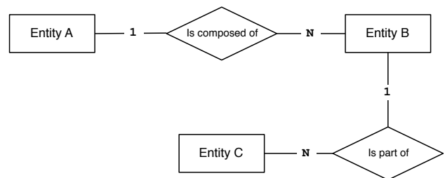
Figure 1: ER Model representing charges, debts and elements.
