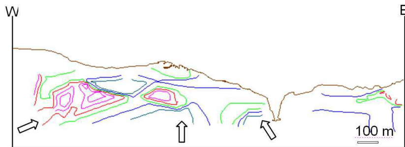
Fig. 3. Ratio \log\text{Ag} / \log\text{Pb} isovalue contours plotted on longitudinal section along the vein. Contour values: 0.9, 1.0, 1.1, 1.2, 1.4. (From chemical data in ppm).
