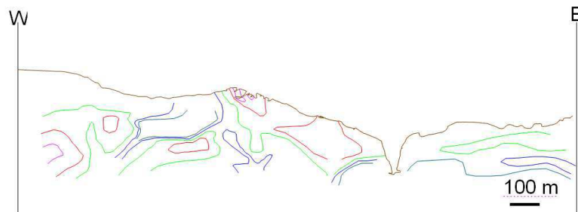
Fig. 1. Ag (logarithm of ppm) isocontent contours plotted on longitudinal section along the vein. Contour values: 2.2, 2.4, 2.6, 2.8, 3.0.
