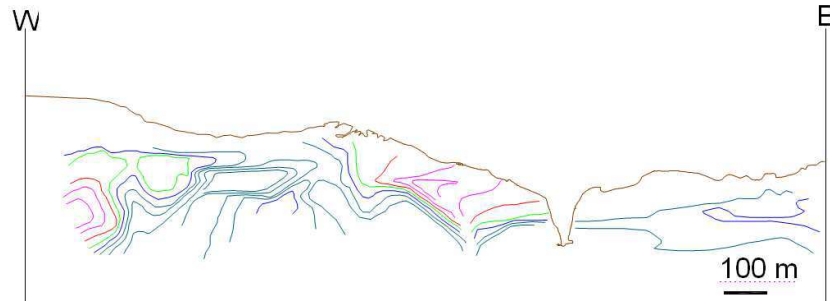
Fig. 2. Factor 1 (log) isovalue contours plotted on longitudinal section along the vein. Contour values: -1.0/0.0, 0.2, 0.4, 0.6, 0.8-1
