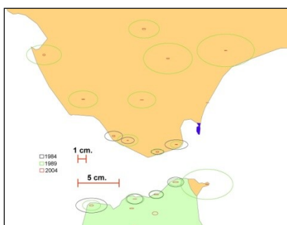
Figure 8 Error ellipses. 1984-2004 works
