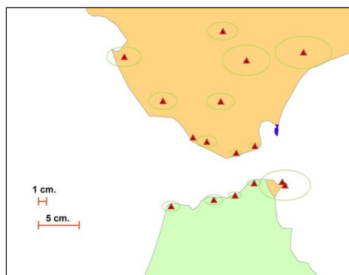
Figure 4 Error ellipses. 1989 works
