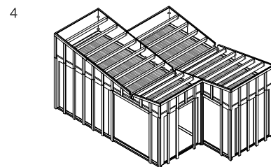
4- Assembly of roof joist.
