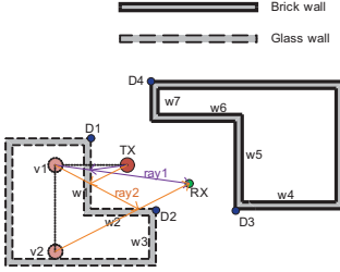
Figure 6 Reflection path searching
