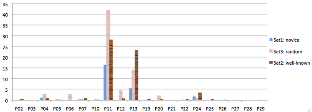
Figure 2: Average number of pitfall/ontology, by set; for P8, the averages are 62, 297, and 303, respectively.
