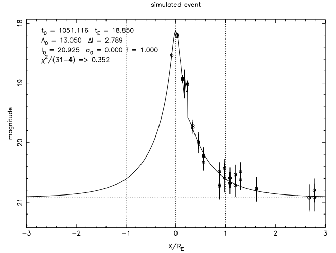
Figure 8. Best-fitting lens + planet model for a simulated light curve which includes a planetary deviation. This gives a lower \chi^2 than Fig. 7, indicating a better fit. The fitted parameters appear in the top left-hand corner of the plot and the planet is at position x/R_E = 1.05 , y/R_E = 0.39 on the lens plane, interfering with one of the major images.
