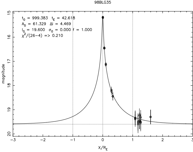
Figure 3. Fitted light curve for microlensing event 98BLG35. R magnitude is plotted versus separation in units of R_E . The estimated event parameters are shown on the top left-hand corner of the plot.
