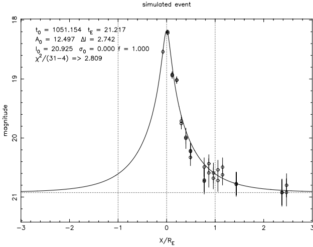
Figure 7. Shown above is the best-fitting single lens model for a simulated light curve which includes a planetary deviation. The fitted parameters appear in the top left-hand corner of the plot. The residuals of the fit are shown in Fig 9. The \chi^2 value improves by a factor of 8 if we allow for the presence of a planet as shown in Fig 8.
