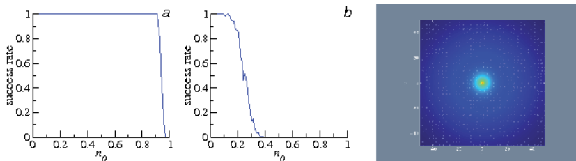
Fig. 3. Panels a and b show the success rate of the robot trials locating the target as a function of the density of obstacles n_o , when it moves in a triangular and square lattice respectively. The right panel shows the density of lattice sites visited by the robot for a square lattice with obstacles.
