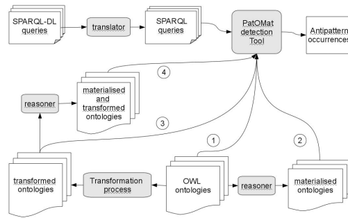
FIG. 1 – The antipattern detection methods
