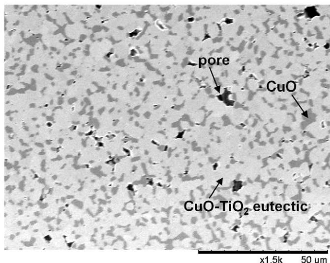
Fig. 4. Surface view by SEM of composition 3 (75% CuO–25% TiO 2 ) thermally treated at 1045 °C in air. The dark phase is CuO and the light phase is the CuO–TiO 2 eutectic.
