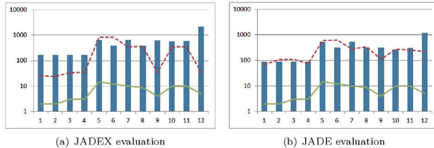
Figure 5: Test code lines (Y axis) per Test Case (X axis) comparison for JADEX (a) and JADE (b)
