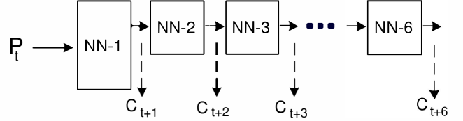
Fig. 2. Structure of Neural Networks for prediction of 1 to 6 hours.
