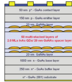
Fig 2 (a) Schematic structure of QDSC with multi-stacked layers of InAs/GaNAs straincompensated QDs.
