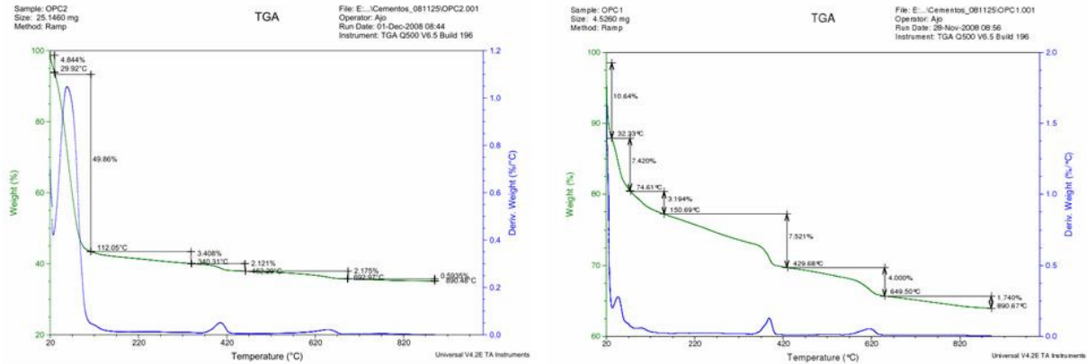
Figure 2: TGA/DTG curves of OPC paste (w/c=0.5) hydrated at 20°C for 3 days (left) and 6 days (right).
