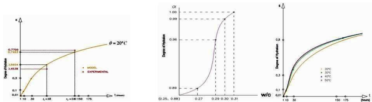
Figure 3: Left: Experimental results and simulation of the evolution of the degree of hydration versus time of an OPC paste (w/c=0.5) at 20°C. Centre: ultimate degree of hydration predicted versus water/cement ratio, at 20°C. Right: Modelled degree of hydration versus time of the same OPC sample, at different temperatures
