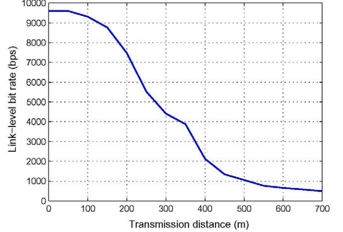
Fig. 7. Hotspot link throughput.
