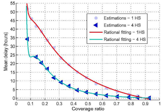
Fig. 12. Localization delay – means and fittings for 1 and 4 hotspots.
