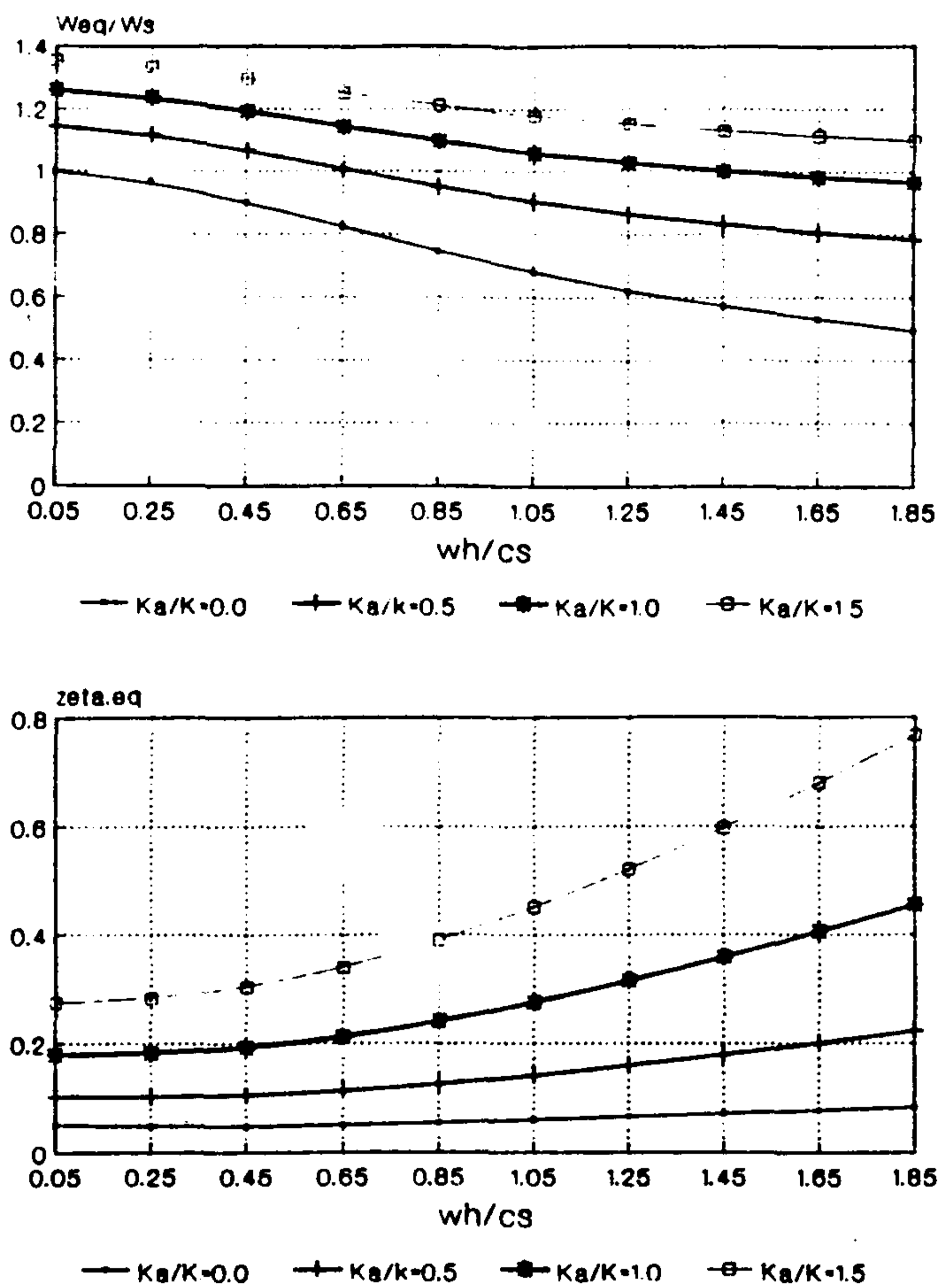
Fig. 5 Equivalent frequency and damping ratio. k_a/k dependence. Built-in pier
