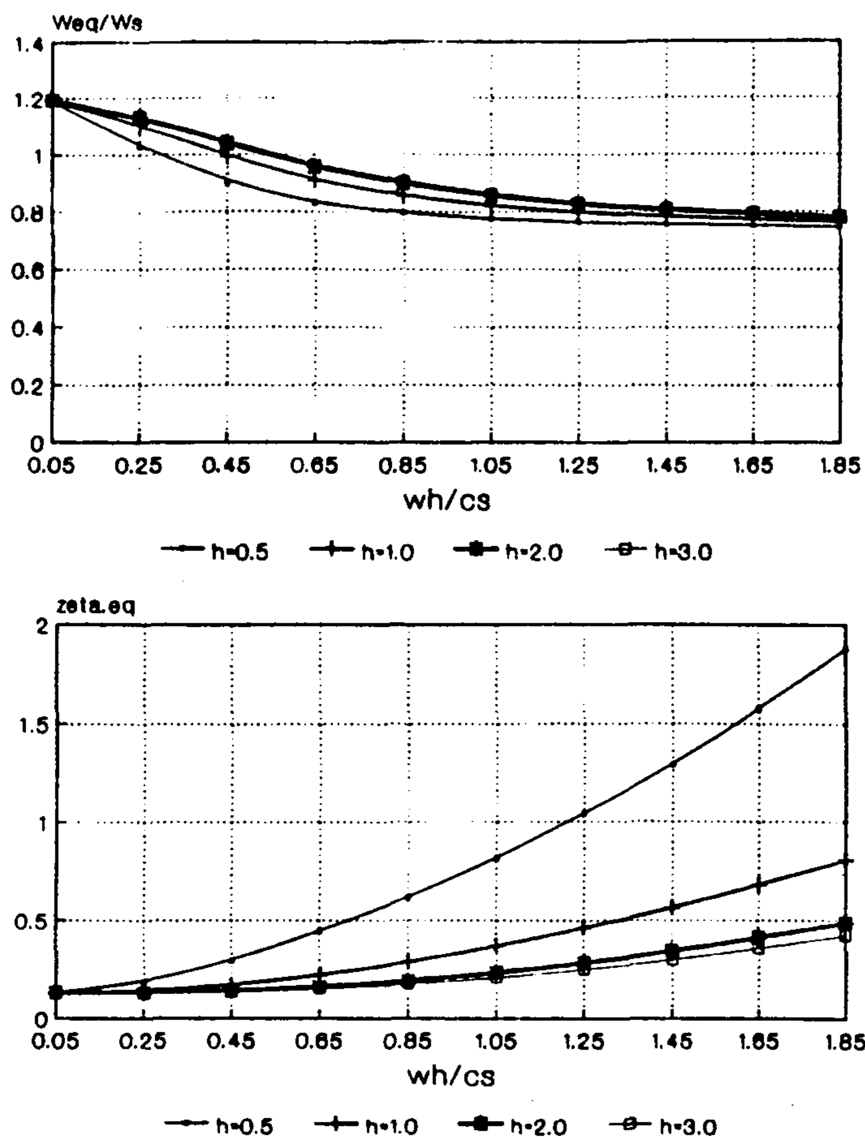
Fig. 2 Equivalent frequency and damping ratio. \bar{h} dependence. Hinged pier.
