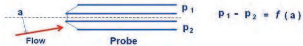
Fig. 3. Vertical cut of three tubes showing the leading edges and the angle determination concept
