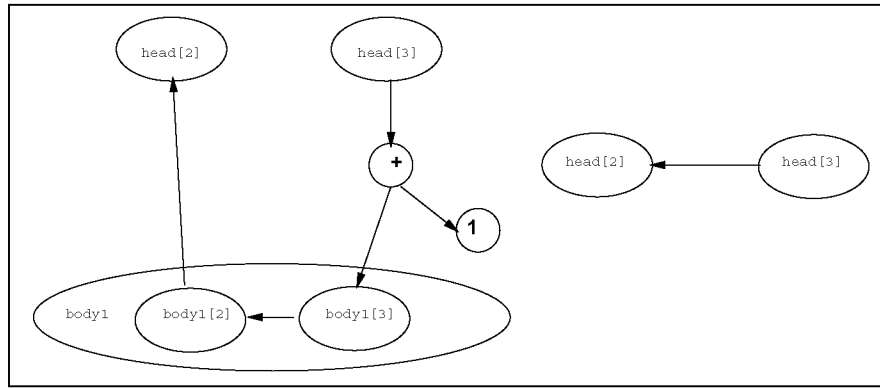
Figure 1: Size dependency graphs for predicate append/3 .
