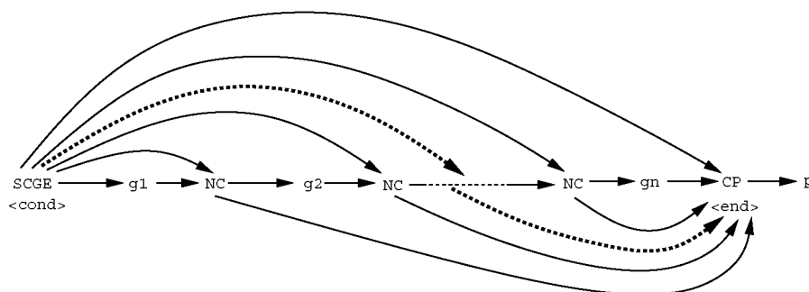
Fig 2: Representing CGE in Goal Chain
