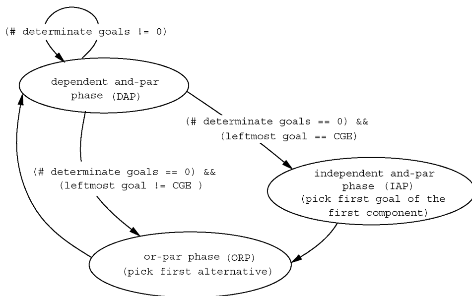
Fig 1: Phases in Parallel Execution
